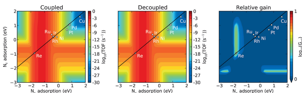
Figure 3. Coupled (left) and decoupled (center) TOF maps and the relative bifunctional gain, G_{rel} (right), for ammonia synthesis, coupling a metal(211) ( s site) and a metal(111) ( t site) facet. The adsorption energies of N on various metals define the scaling relation between adsorption on the two facets (black line), which would act as a constraint in the case where the two catalytic sites are composed of the same metal or alloy.
